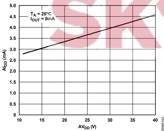
Figure 9. A_{DD} vs. AV_{DD}
