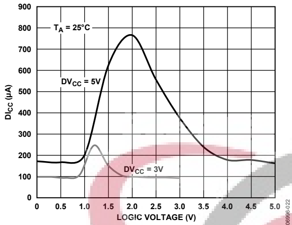
Figure 7. D_{CC} vs. Logic Input Voltage
